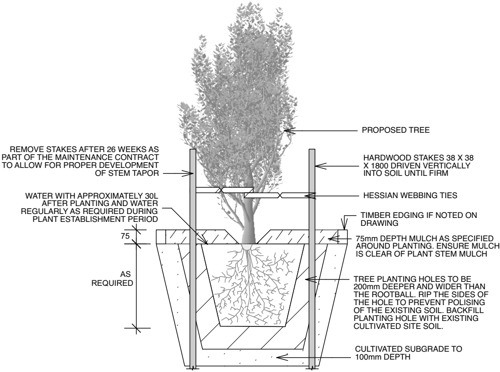
TREE PLANTING & STAKING DETAIL SCALE 1:20
